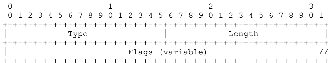
Figure 11: Prefix Attribute Flags TLV Format
