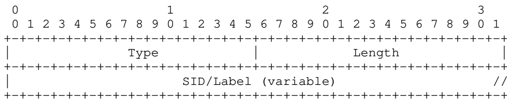
Figure 2: SID/Label TLV Format
