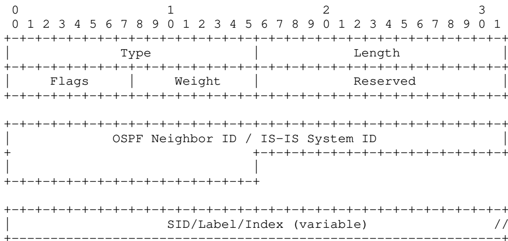
Figure 8: LAN Adjacency SID TLV Format
