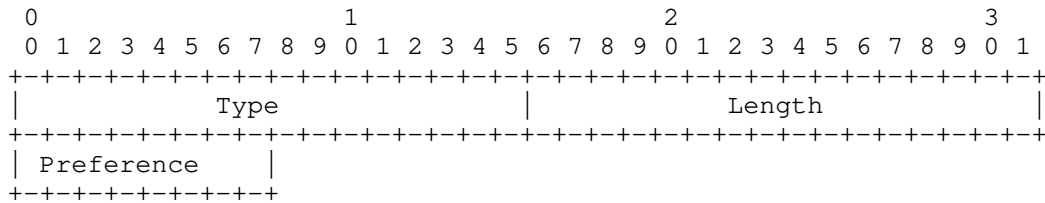
Figure 6: SRMS Preference TLV Format
