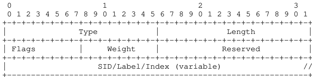
Figure 7: Adjacency SID TLV Format
