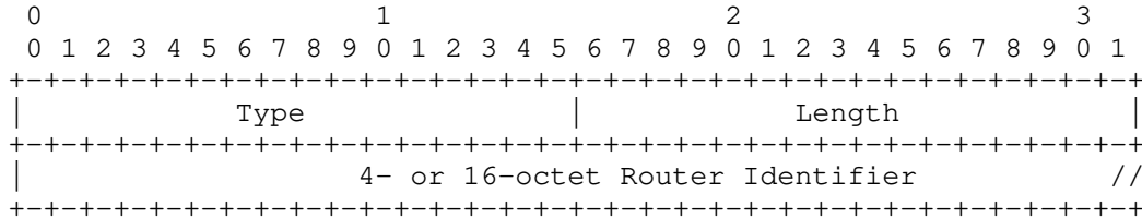
Figure 12: Source Router Identifier TLV Format
