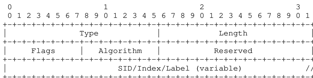
Figure 10: Prefix-SID TLV Format
