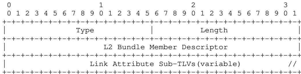
Figure 9: L2 Bundle Member Attributes TLV Format
