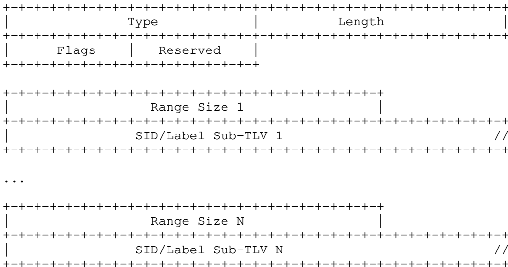
Figure 3: SR Capabilities TLV Format
