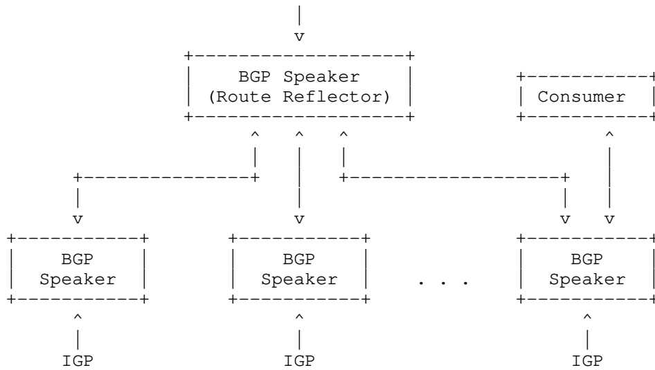
Figure 1: Link-State Information Collection
